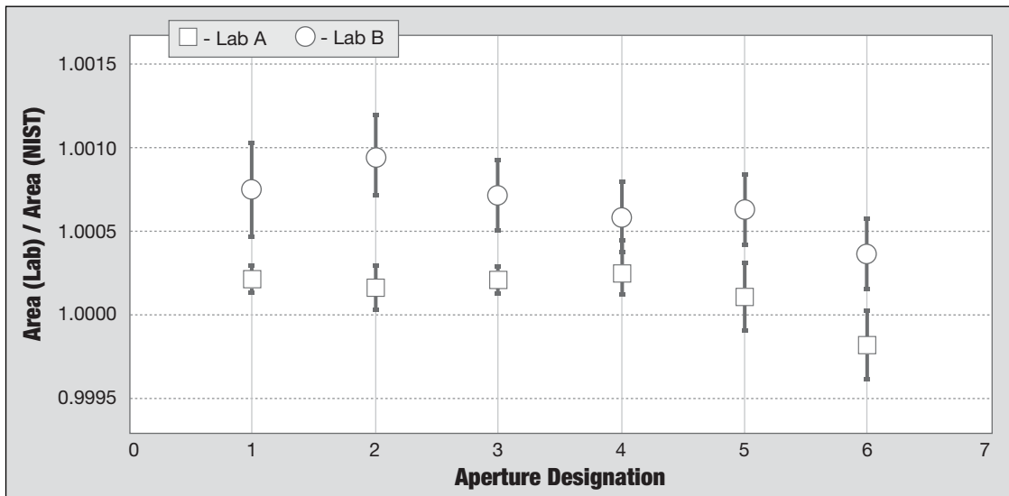
Figure 5. Results of a round-robin aperture-area comparison, showing preliminary calibration results on six aperture measurements made at two laboratories. Results are shown as the ratio of the laboratory area to the area measured by NIST. The vertical lines correspond to the combined expanded uncertainties.
