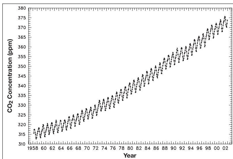
Figure 1. Atmospheric carbon dioxide monthly mean mixing ratios as observed by Tans and Keeling at Mauna Loa, Hawaii. Data prior to May 1974 are from the Scripps Institution of Oceanography, and data since May 1974 are from the National Oceanic and Atmospheric Administration (NOAA).
